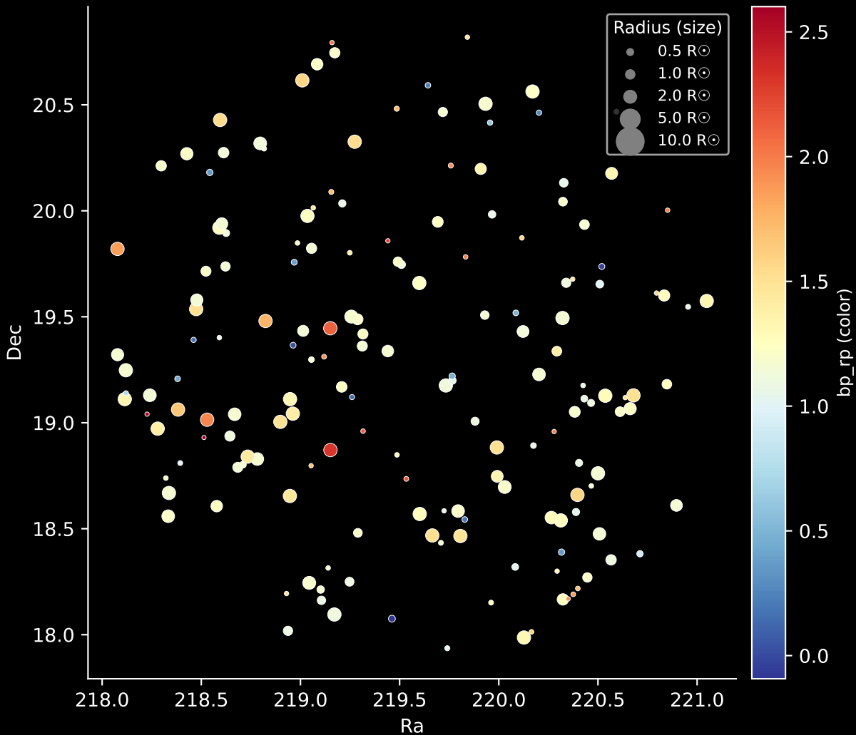
APOGEE DR17 Field: [202+23_MGA] Stars: 172
