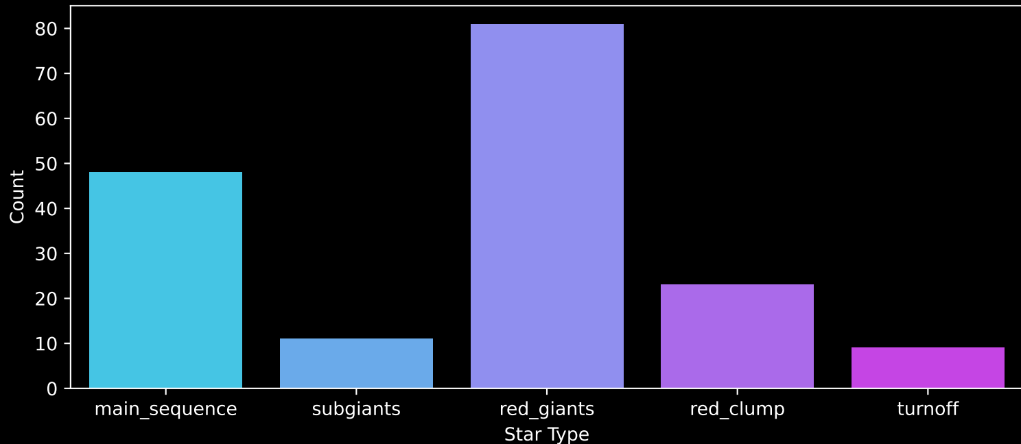
APOGEE DR17 Field: [202+23_MGA] Count plot of Star Type
