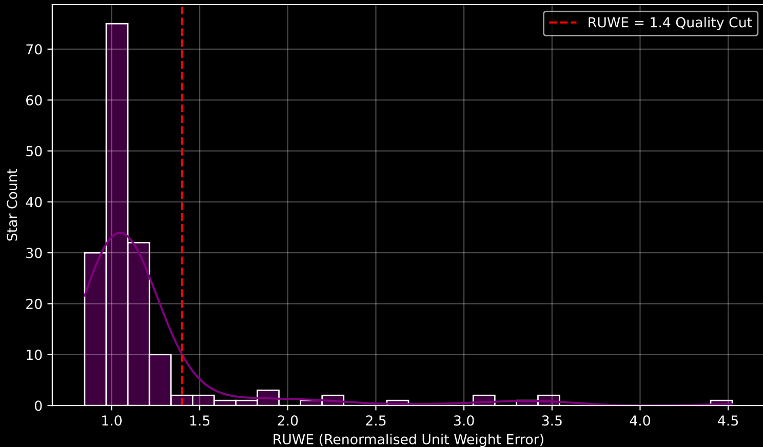
GAPOGEE DR17 Field [202+23_MGA] RUWE Distribution (n= 166)
