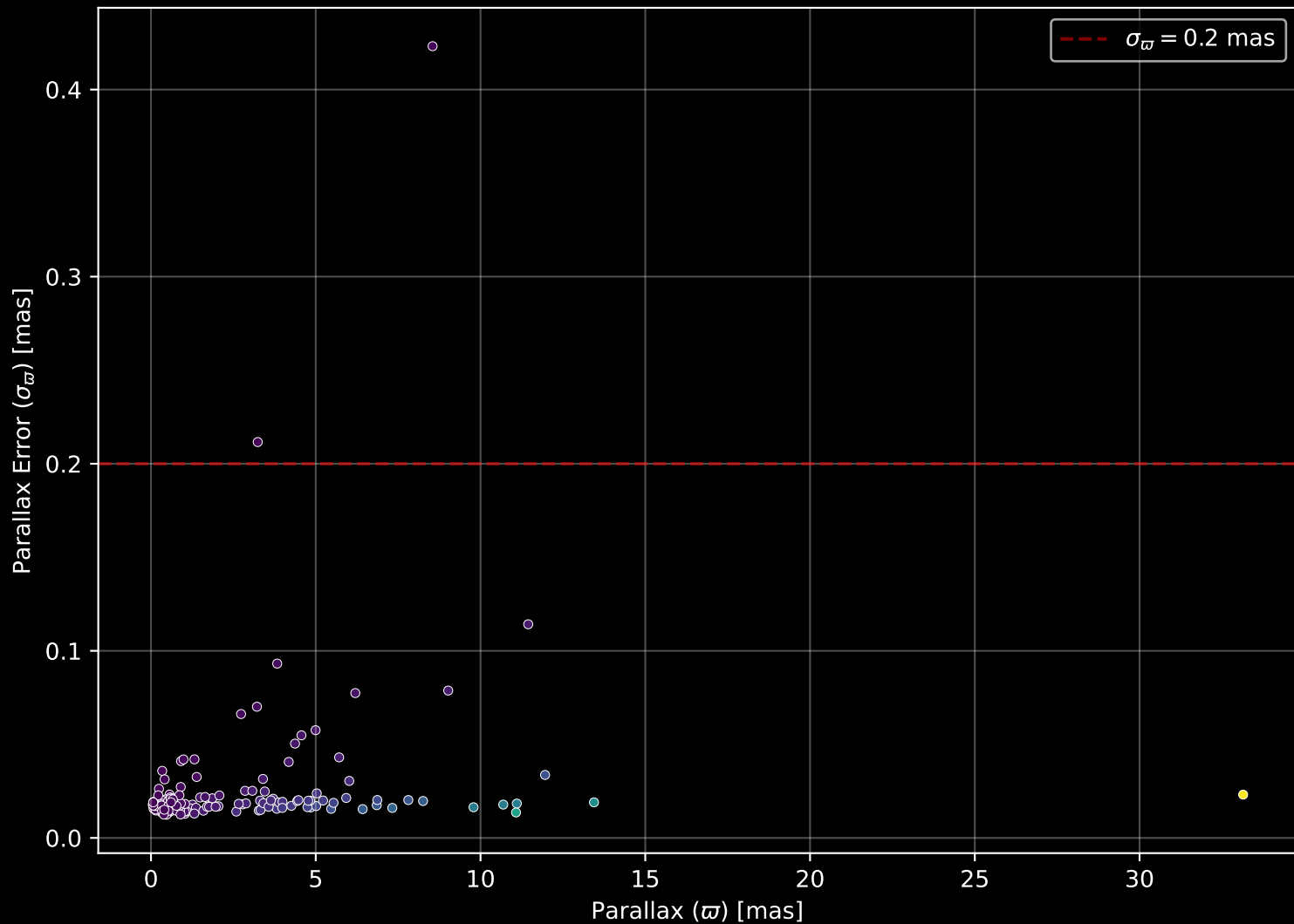
APOGEE DR17 Field: [202+23_MGA] Parallax Quality (n= 172)
