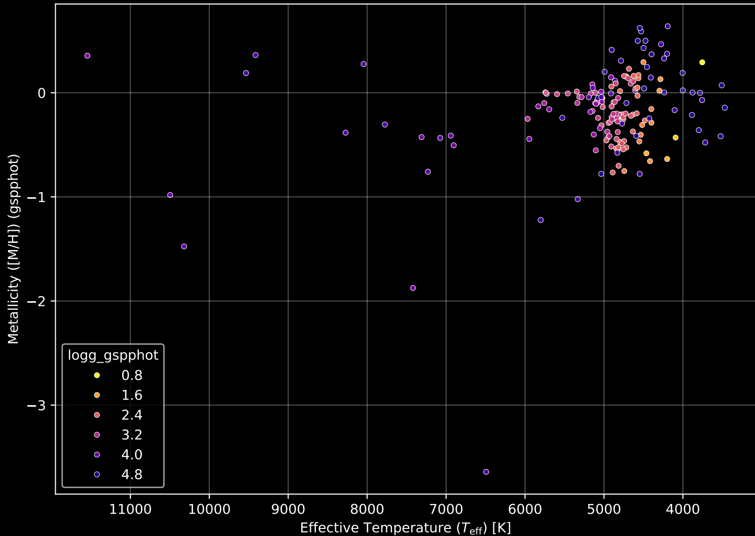
APOGEE DR17 Field: [202+23_MGA] Stellar Population Parameters (n= 172)
