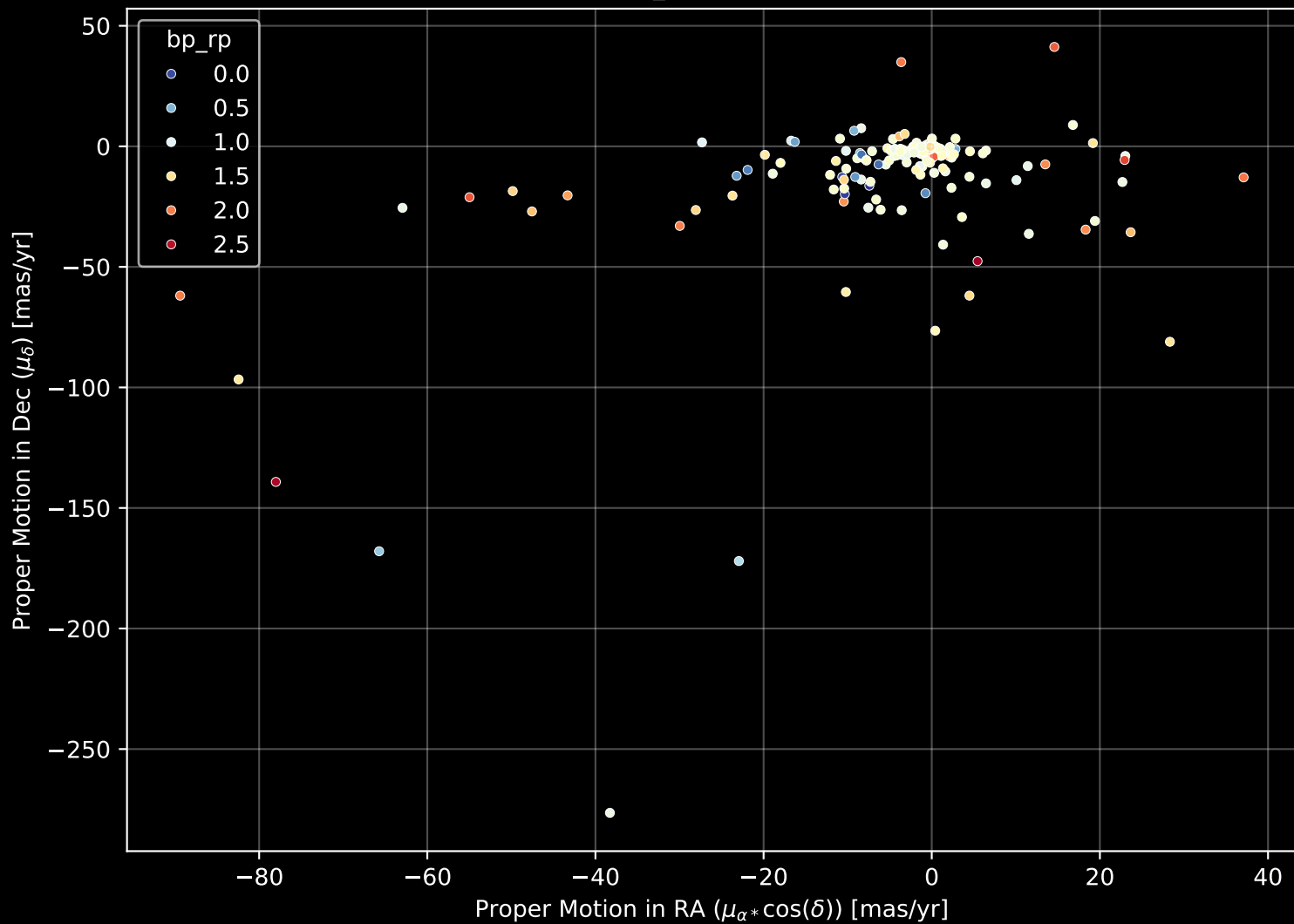
APOGEE DR17 Field: [202+23_MGA] Proper Motion Diagram (n= 172)
