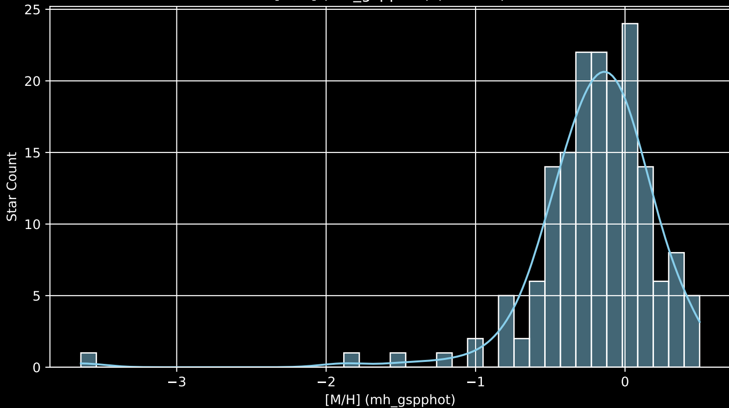
APOGEE DR17 Field: [202+23_MGA [M/H] (mh_gspphot) (n= 169)
